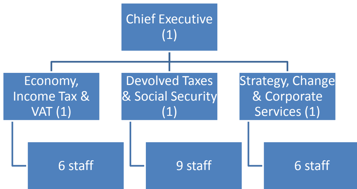
Figure 3: Organogram
